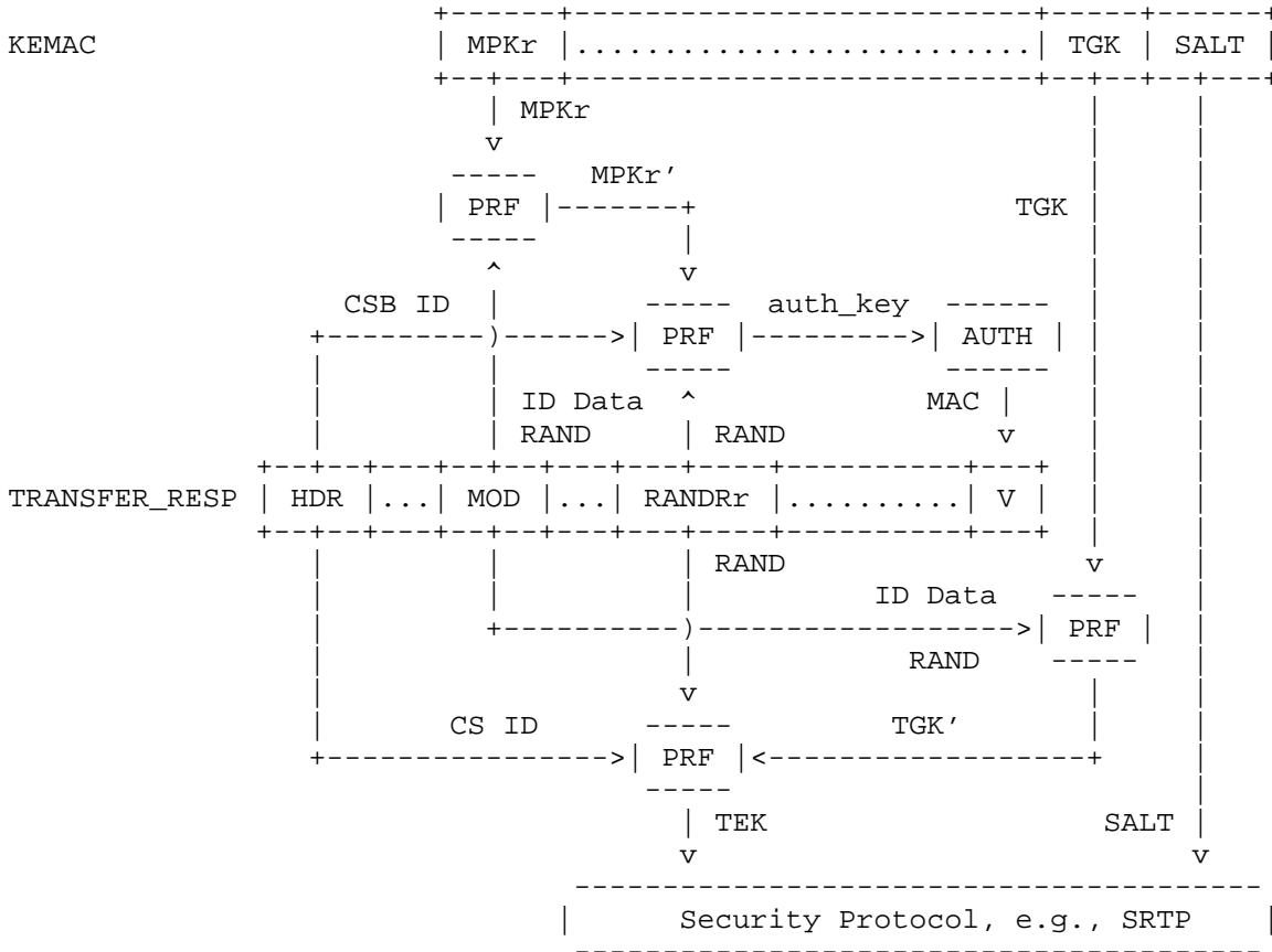
Figure 5: Key hierarchy with key forking and RANDRr
