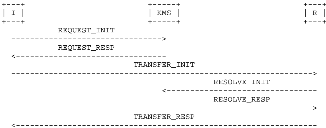
Figure 1: Full three round-trip signaling
