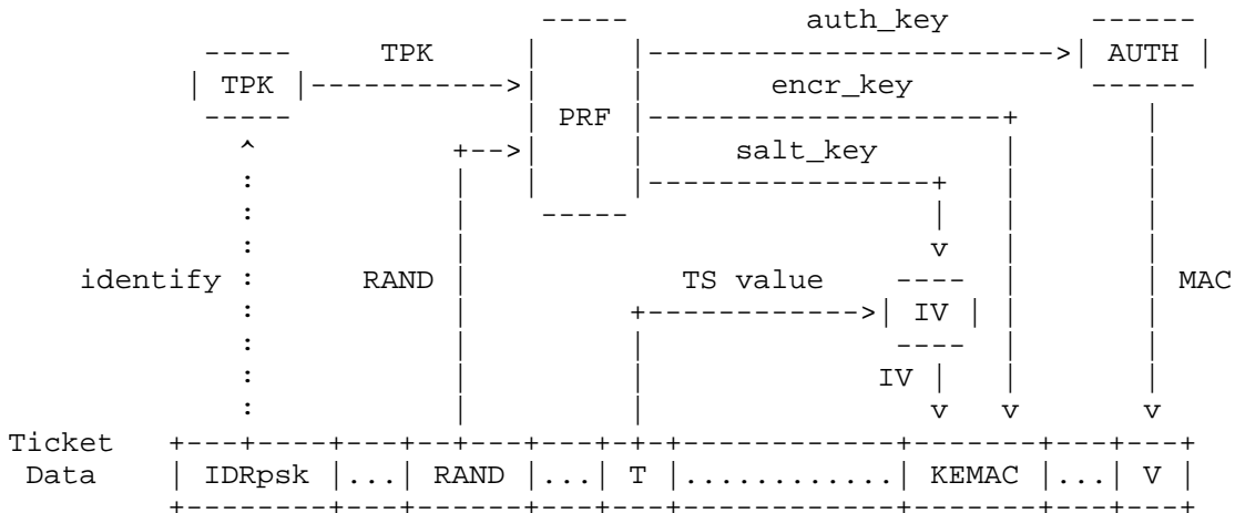
Figure 10: Deriving keys from a TPK
