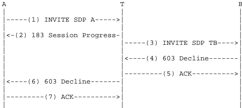
Figure 3: Unsuccessful session establishment
