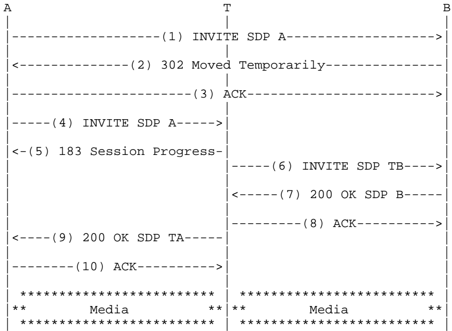
Figure 4: Callee's invocation of a transcoder
