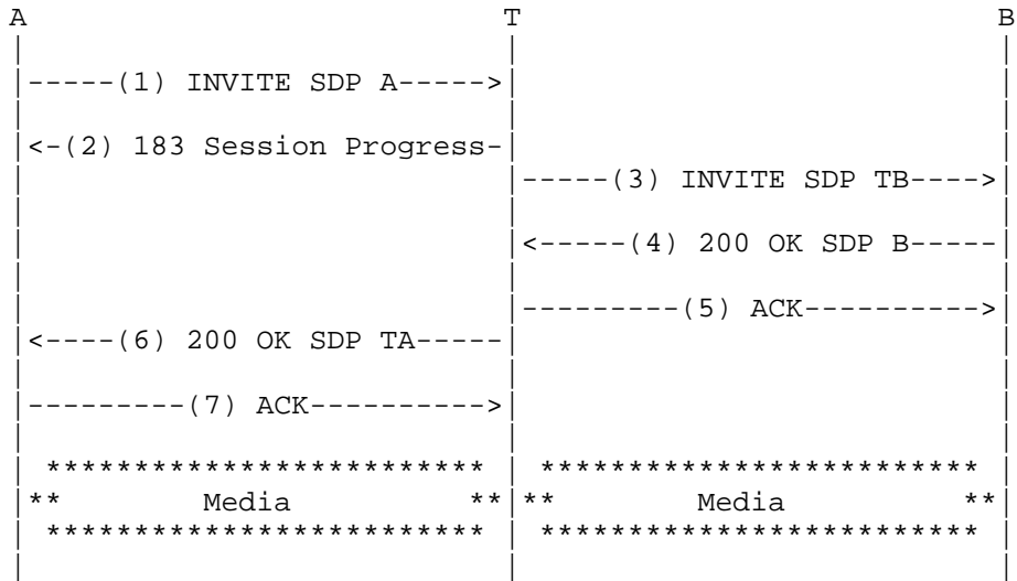
Figure 2: Successful invocation of a transcoder by the caller
