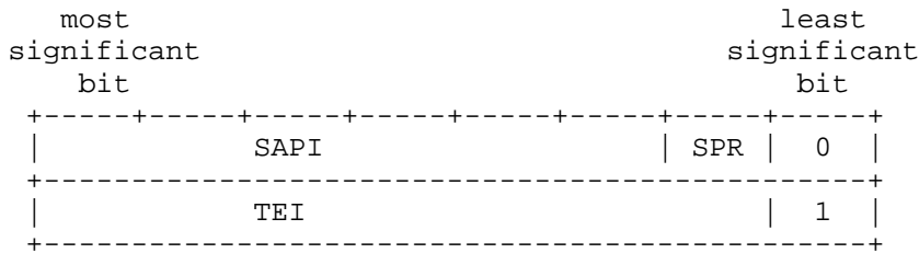
Figure 5. DLCI Format
