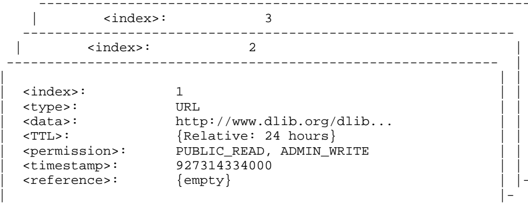
Figure 3.1: Handle "10.1045/may99-payette" and its set of values
