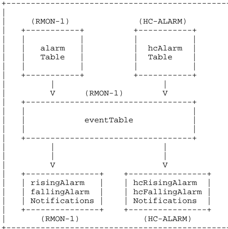
Figure 1: HC-ALARM MIB Functional Structure
