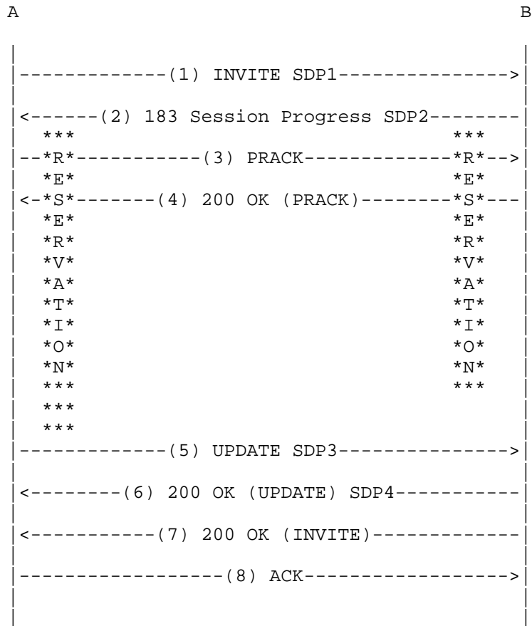
Figure 3: Session modification with preconditions
