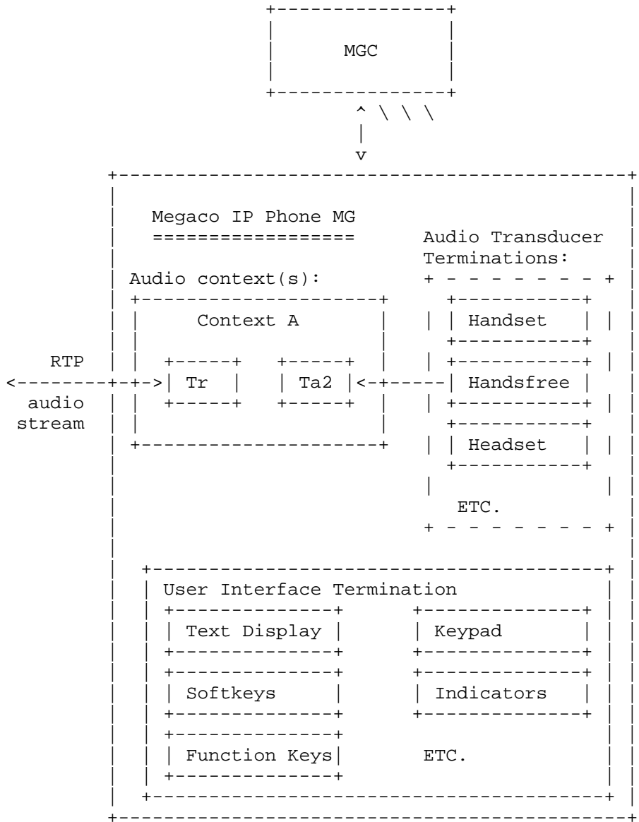
Figure 1: Megaco IP Phone Termination / Package Model
