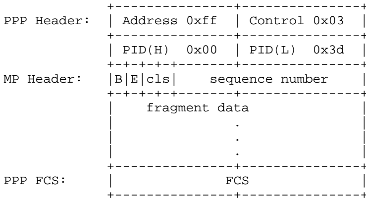
Figure 2: Short Sequence Number Fragment Format With Classes
