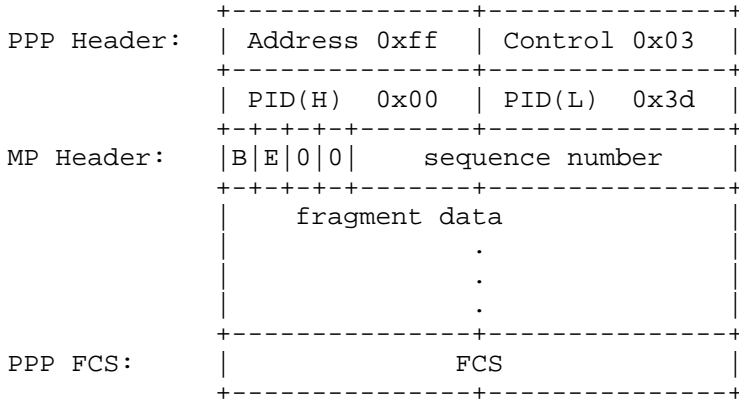
Figure 1: Multilink Short Sequence Number Fragment Format [2]
