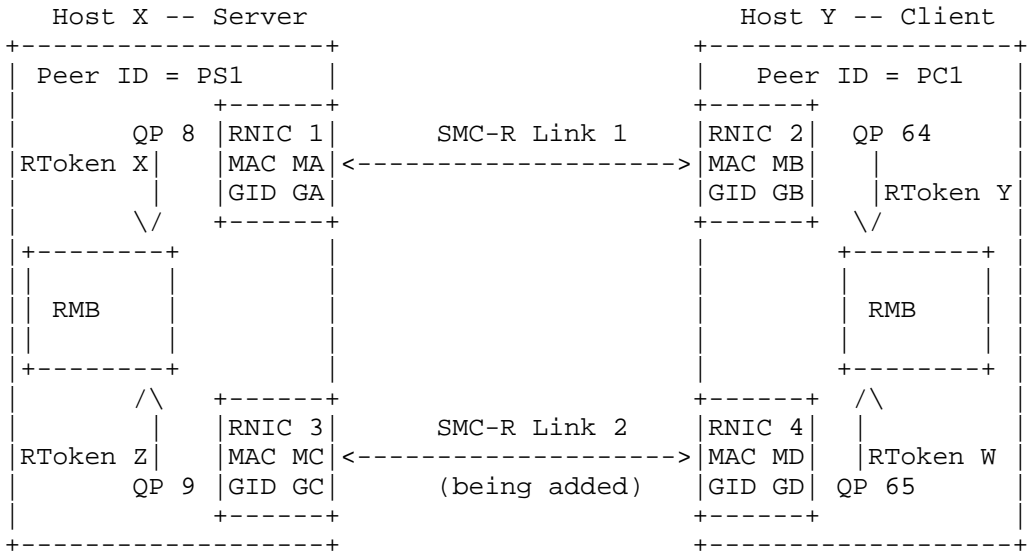
First SMC-R link setup as shown in Figure 8
