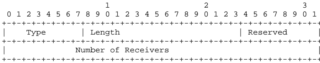
Figure 18: Multicast Receiver Port Count TLV
