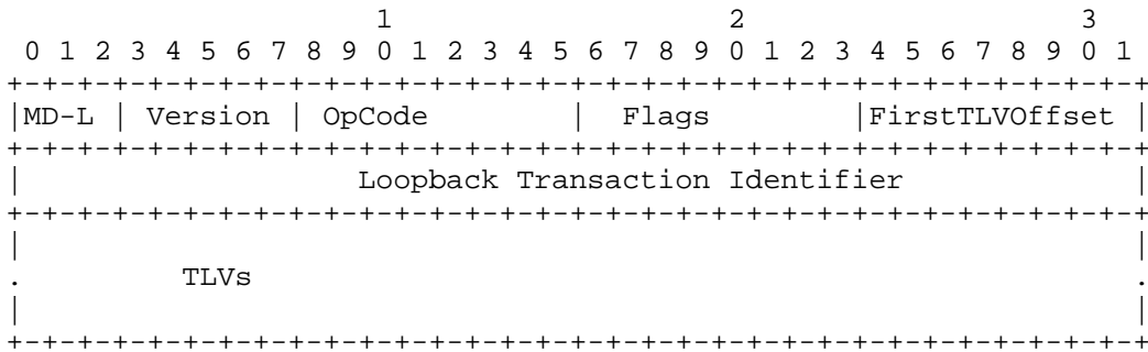
Figure 23: Loopback Message Format
