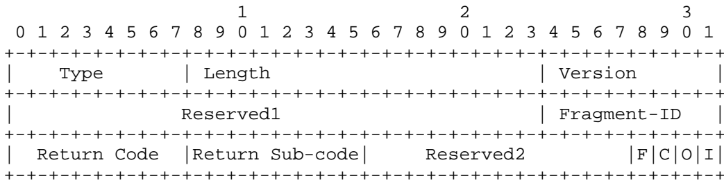
Figure 11: TRILL OAM Application Identifier TLV
