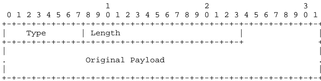
Figure 14: Original Data Payload TLV
