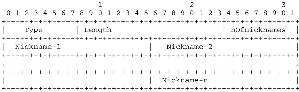
Figure 15: RBridge Scope TLV
