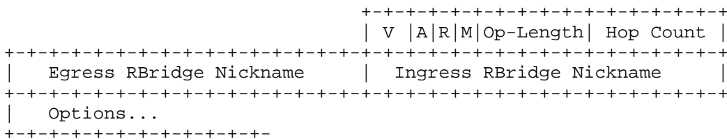
Figure 2: TRILL Header with the "A" Flag
