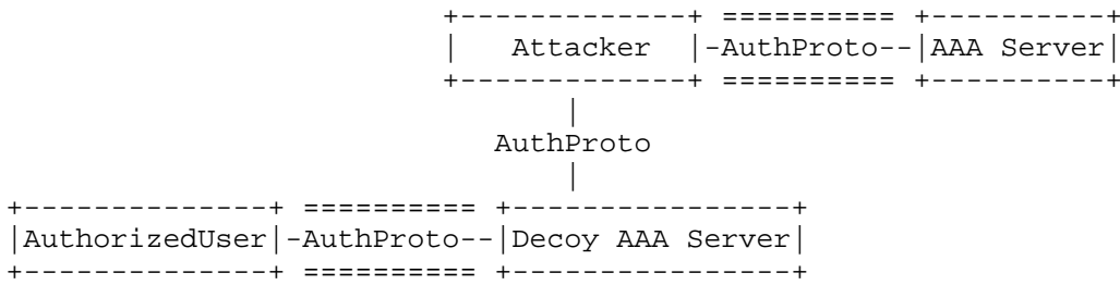
Figure 1: One Example of Original Asokan Attack
