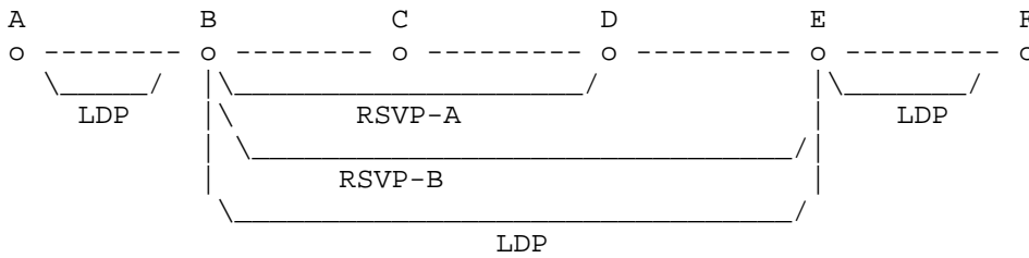
Figure 8: Hierarchical LSPs
