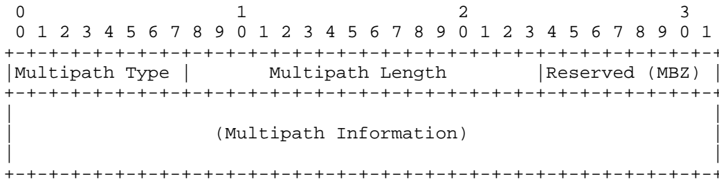
Figure 4: Multipath Sub-TLV
