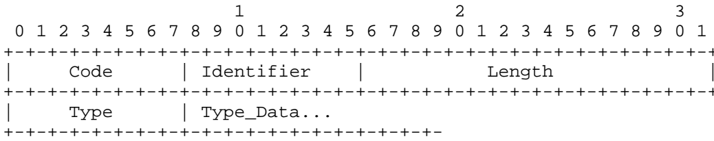
Figure 25: EAP Message Format
