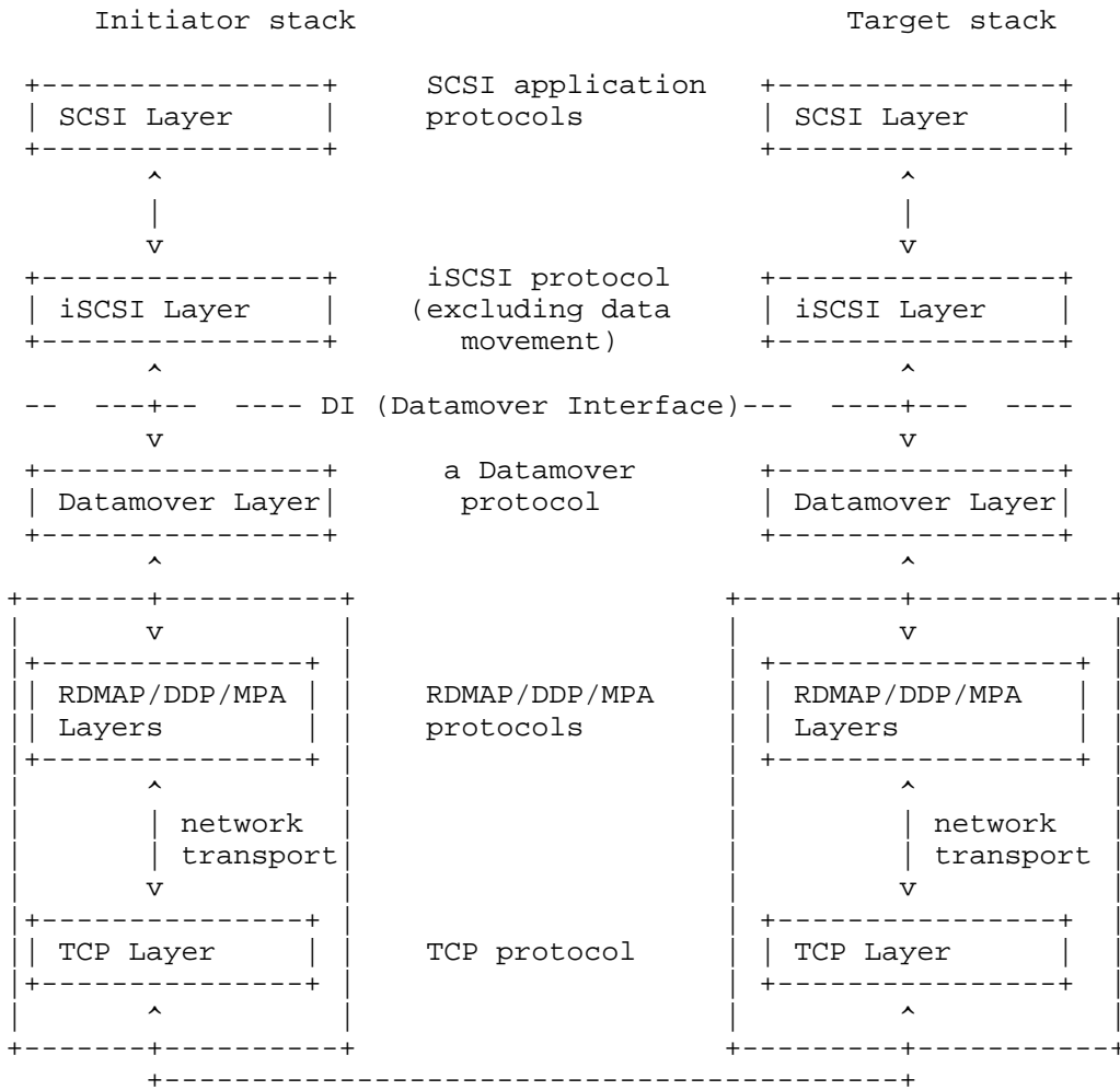
Figure 1. Datamover Architecture Diagram, with the RDMAP Example
