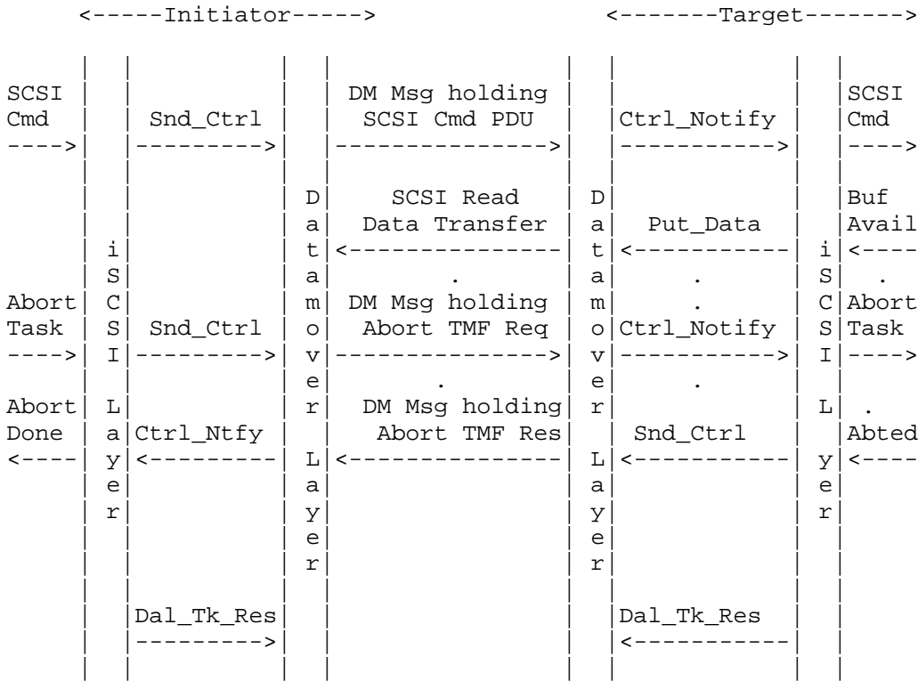
Figure 12. Task Resource Cleanup on Abort
