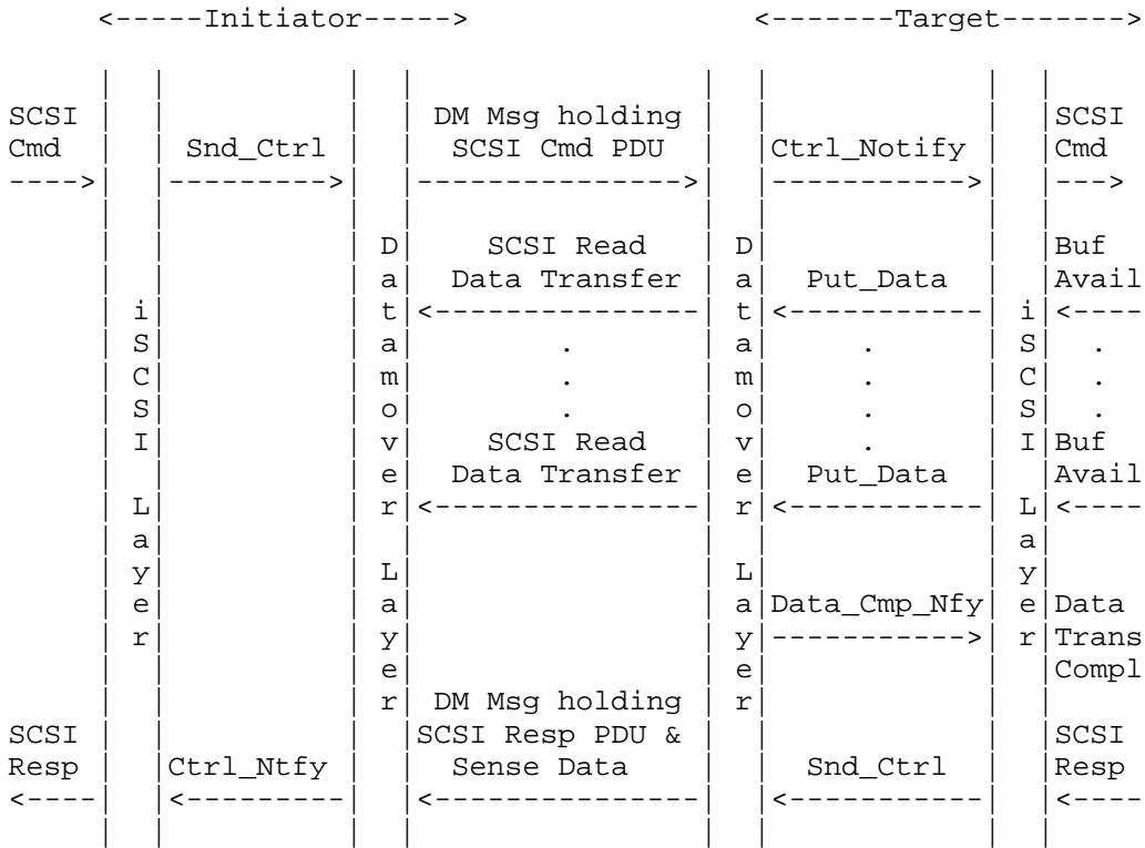
Figure 10. A SCSI Read Data Transfer
