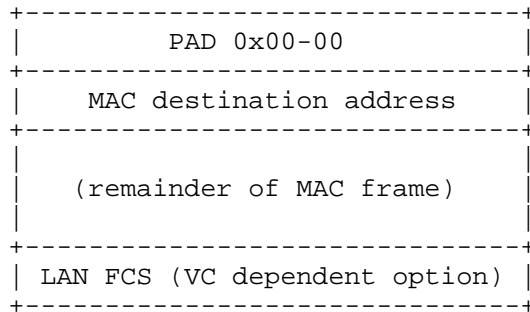
Payload Format for Bridged Ethernet/802.3 PDUs
