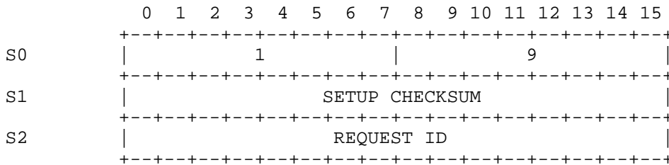
DELETE ALL STREAMS REQUEST Figure 14
