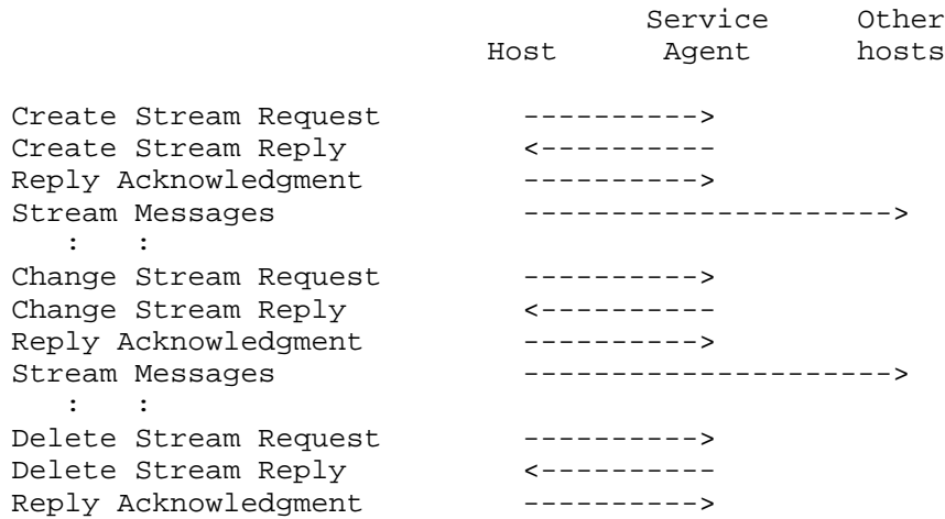
STREAM EXAMPLE Figure 7
