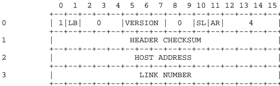
RESTART COMPLETE Figure 38
