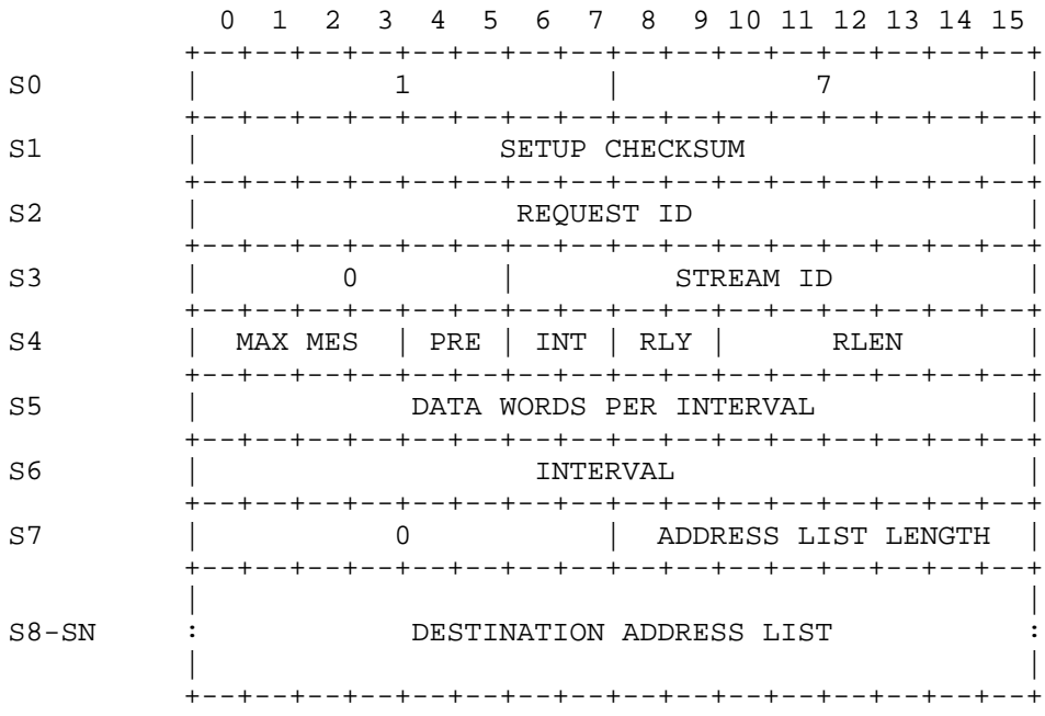
CHANGE STREAM REQUEST Figure 10
