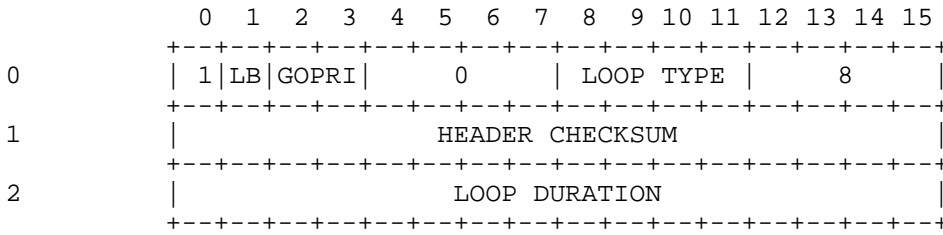
LOOPBACK REQUEST Figure 39
