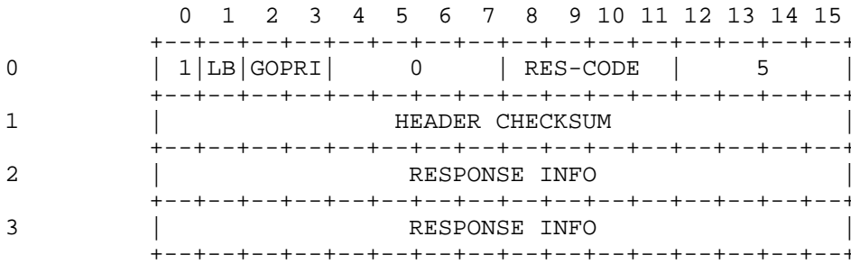
UNNUMBERED RESPONSE Figure 5
