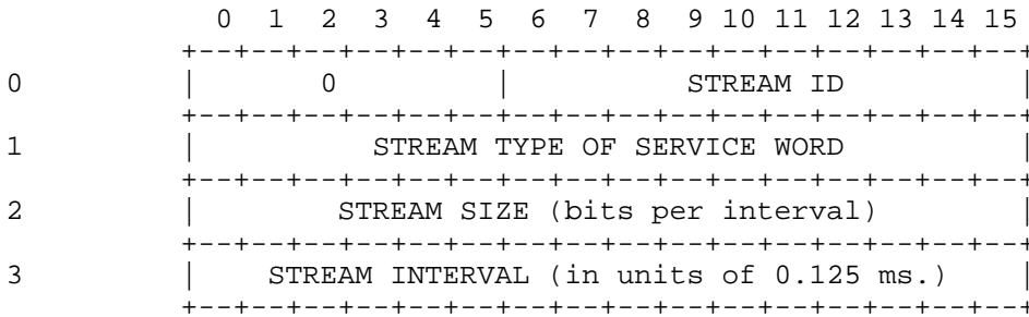
STREAM INFORMATION Figure 33
