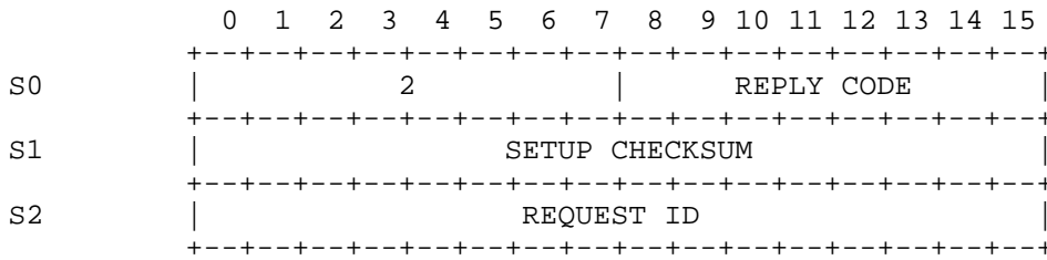
DELETE STREAM REPLY Figure 13
