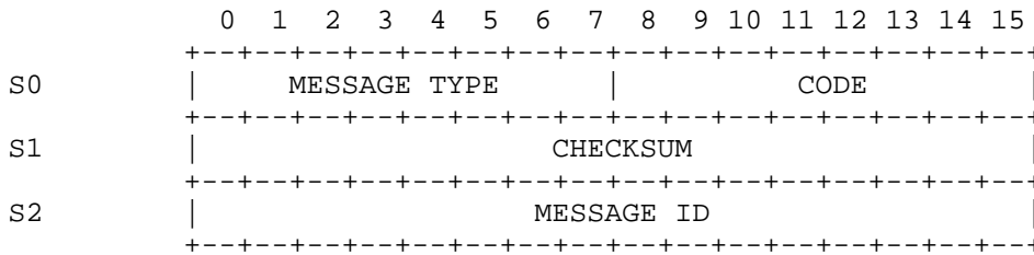
SERVICE AGENT HEADER Figure 6
