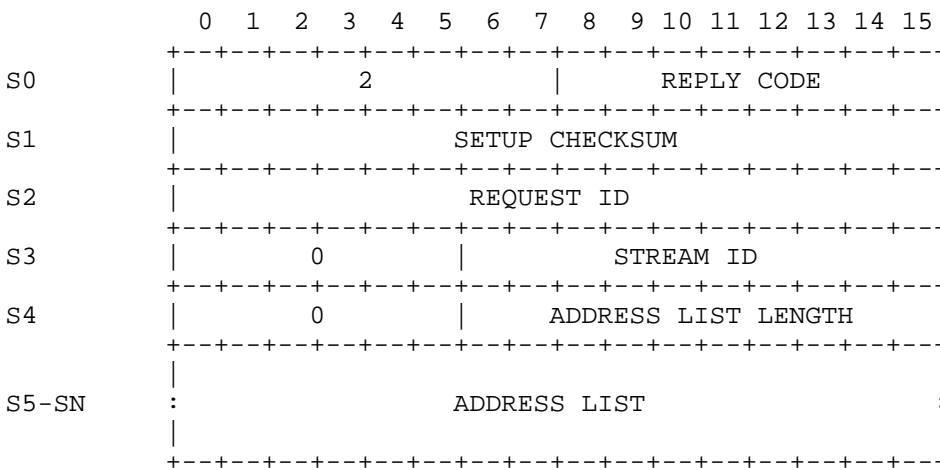
CREATE STREAM REPLY Figure 9
