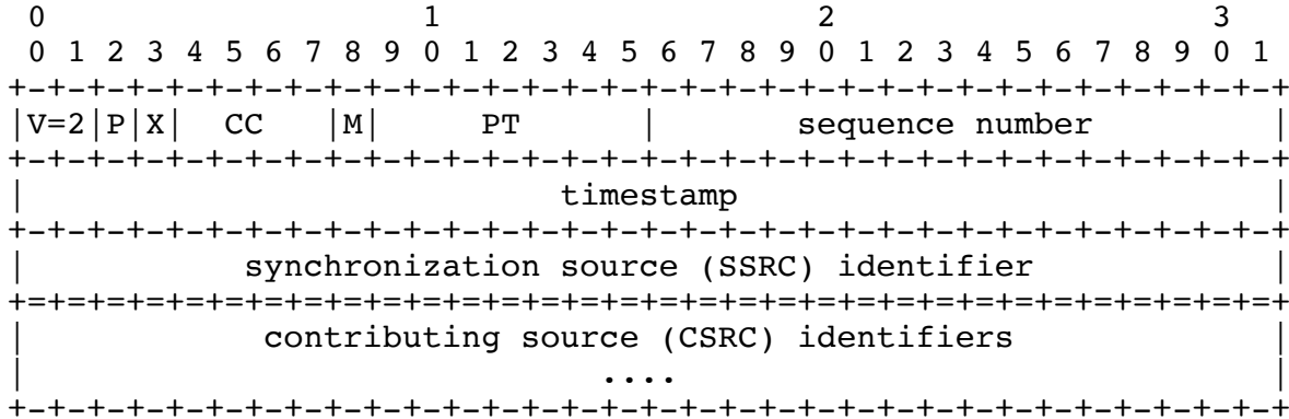
RTP Header According to {{RFC3550}}
