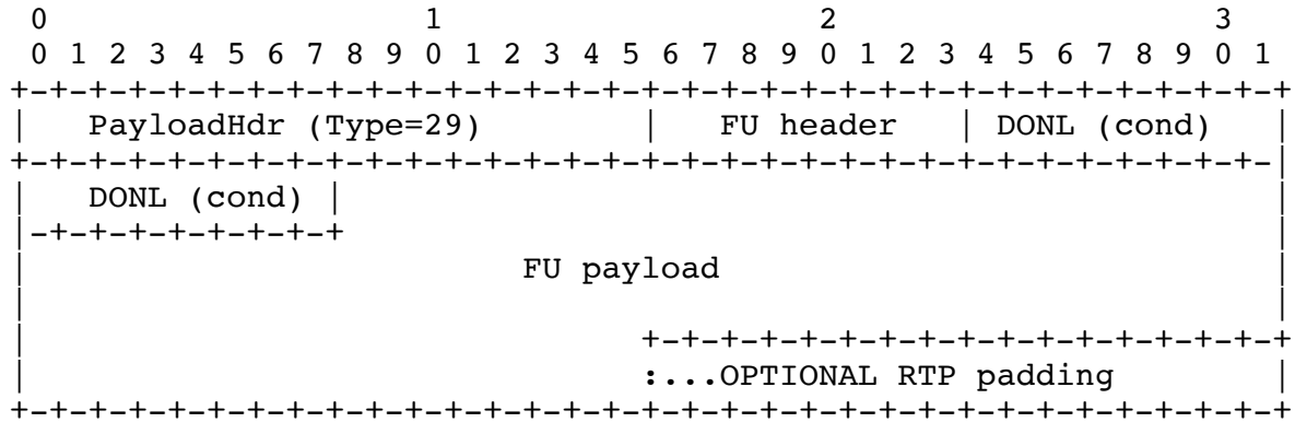
The Structure of an FU
