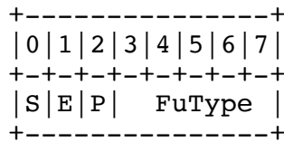
The Structure of FU Header
