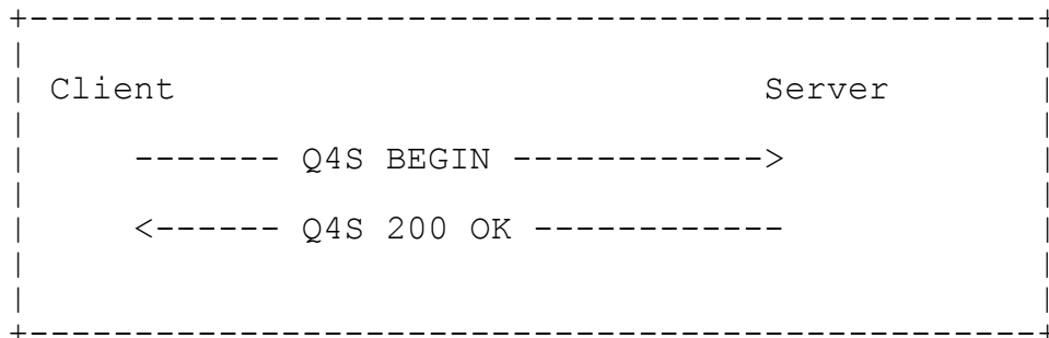
Figure 7 Handshake phase.
